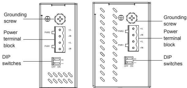
Figure 2 Top Panel
