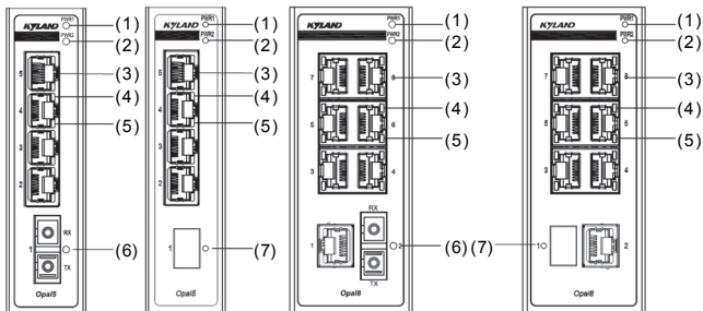
Figure 1 Front Panel
