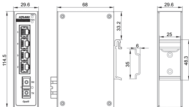
Figure 3 Opal5 Dimensions for DIN-Rail Mounting (unit: mm)
