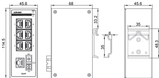
Figure 4 Opal8 Dimensions for DIN-Rail Mounting (unit: mm)
