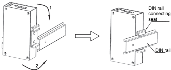
Figure 5 DIN-Rail Mounting
