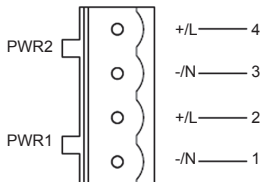
Figure 13 4-Pin 5.08mm-Spacing Plug-in Terminal Block (socket)
