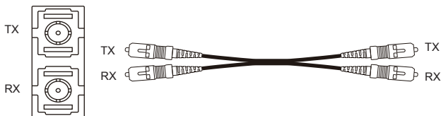
Figure 9 Connection of 100Base-FX Ethernet Port
