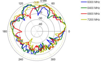
Elevation: 6000 – 7200 MHz
