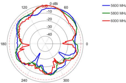
Azimuth: 5600 – 6000 MHz
