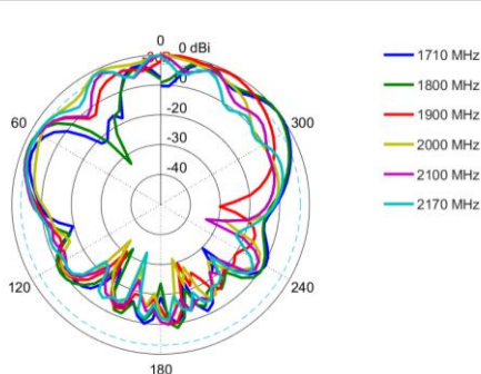
Elevation 1: 1710 – 2170 MHz
