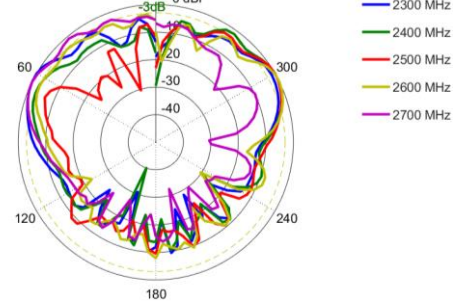
Elevation 2: 2300 – 2700 MHz
