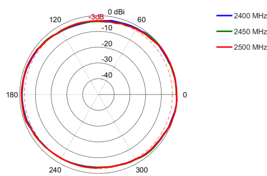
Azimuth: 2400 – 2500 MHz
