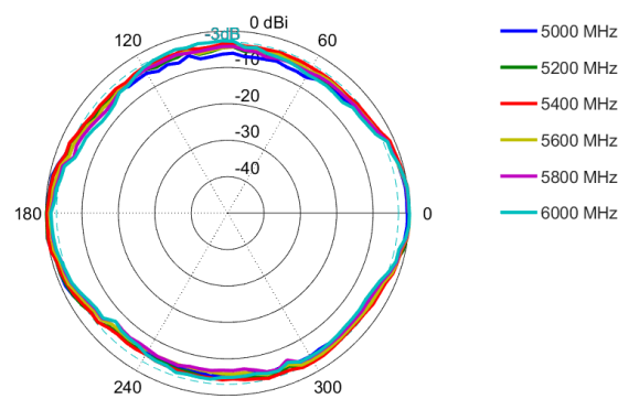
Azimuth: 5000 – 6000 MHz
