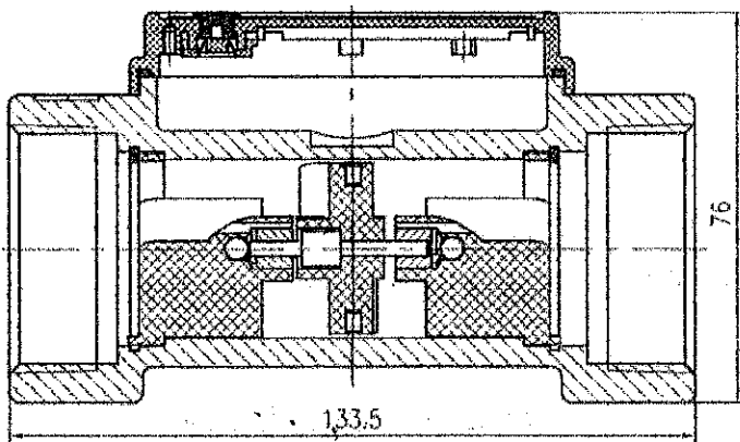
WLL40 Assembly drawing
