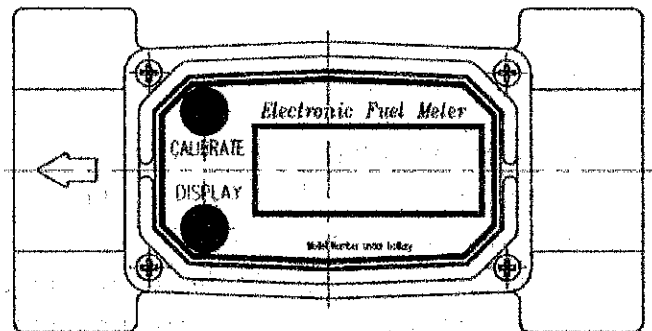
WLL40 Assembly drawing
