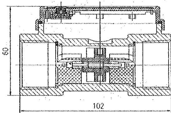
WLL1 Assembly drawing
