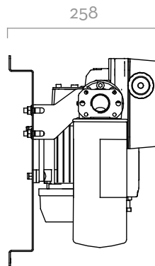
Dimensions expressed in millimeters
