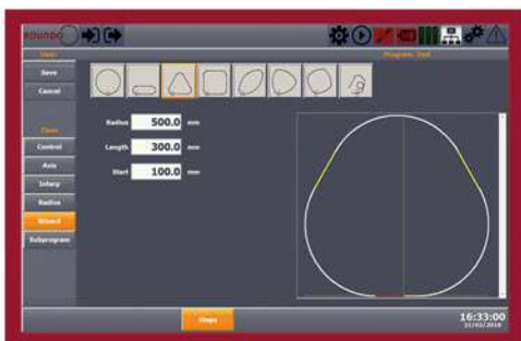
NEW ROUND0 RLC/1 Portable control with joysticks and display
