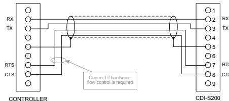
"STRAIGHT" RS-232C SERIAL CABLE
