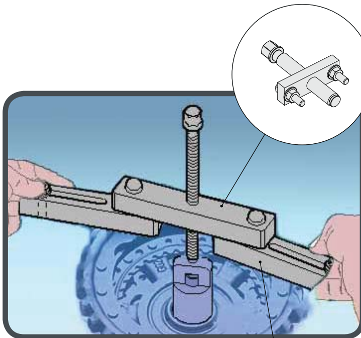
⇧ Assembly of components and tool application.
