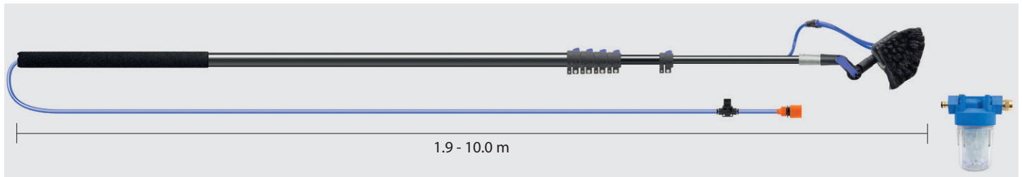
Aluminum telescopic wand with 5 clip fasteners and soft grip (570 mm). High-low shape washing brush with nylon hair on an adjustable angle joint, 12 m hose Ø 8 mm, ball valve and universal connection. 5" filter and filter insert polyphosphate with connection 3/8" coupling and tap connector.
