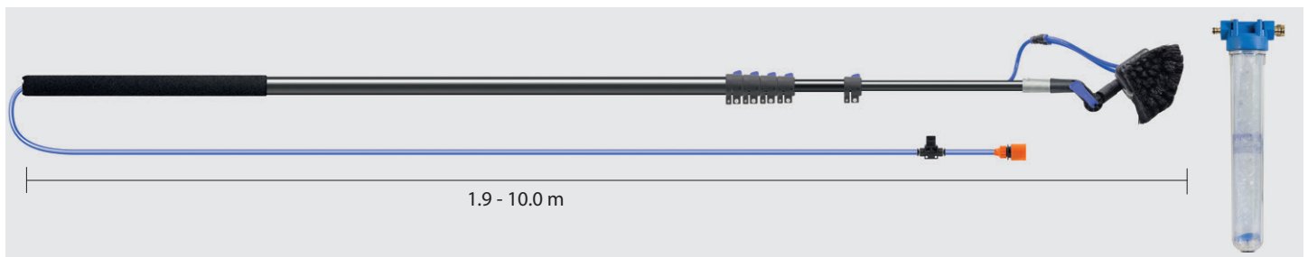
Aluminum telescopic wand with 5 clip fasteners and soft grip (570 mm). High-low shape washing brush with nylon hair on an adjustable angle joint, 12 m hose Ø 8 mm, ball valve and universal connection. 20" filter and filter insert polyphosphate with connection 3/8" coupling and tap connector.
