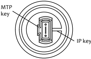
VIEW TO CONNECTOR MPO FEMALE
