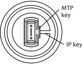
VIEW TO CONNECTOR MPO MALE
