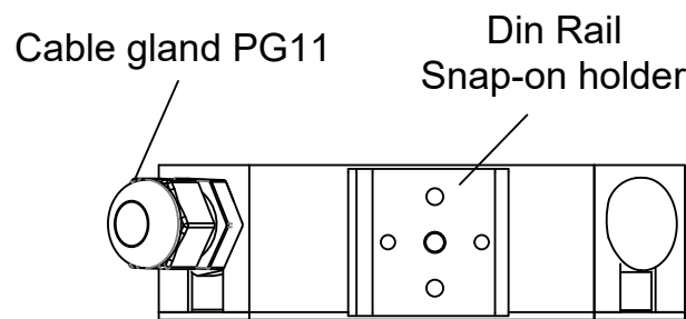
BASIC DIMENSION (BACK VIEW)
