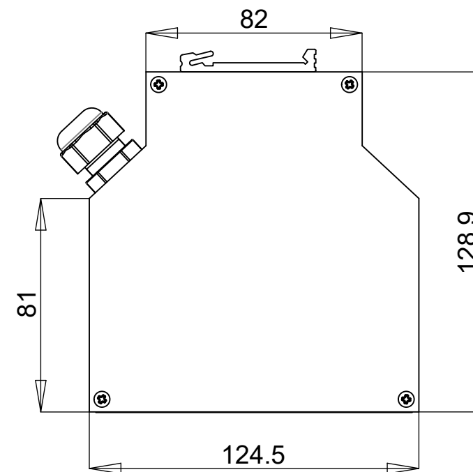
BASIC DIMENSION (TOP VIEW)
