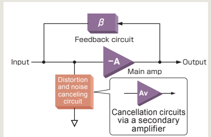
Block diagram of ANCC
