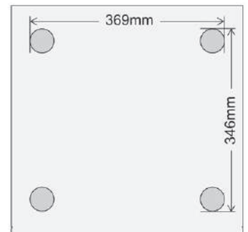
Insulator position / dimensions
