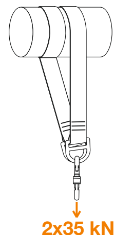
Example of a temporary anchor point
