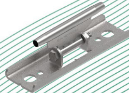
Fig. 27: Intermediate anchor, type: AIO-SZH-14
