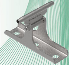
Fig. 25: Intermediate anchor, type: AIO-SZH-11
