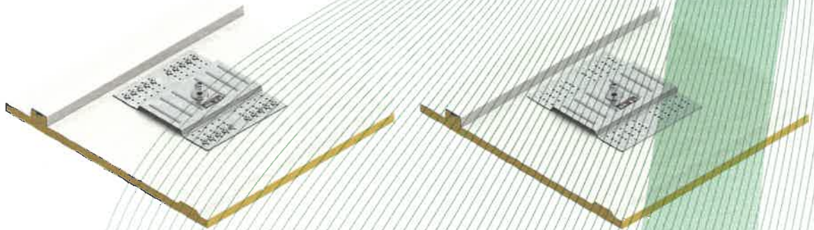
Fig. 1 – 2: Anchor device type A, type SAND-13
