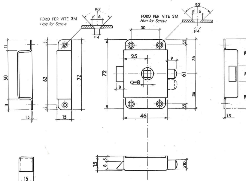
Disegnata serratura interna Drawn inside lock
