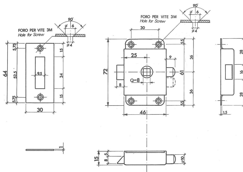
Disegnata serratura interna Drawn inside lock
