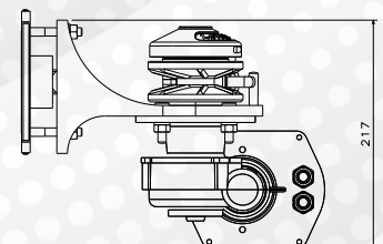
Starboard mounting
