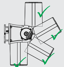
The motor can be installed in various positions.
