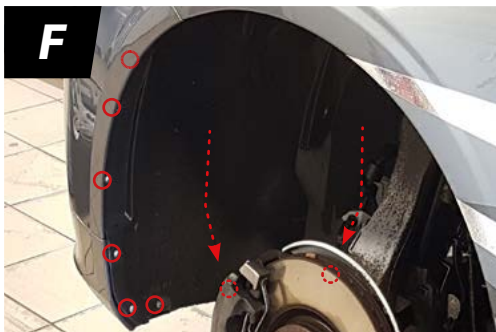
Screws holding the wheelhouse cover.
