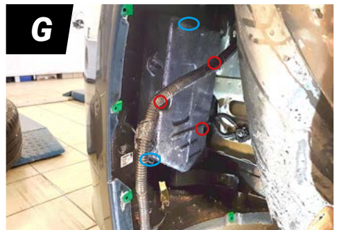
ECM box in wheelhouse.
