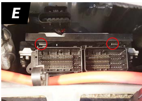
Lockinghooks holding the ECM.
