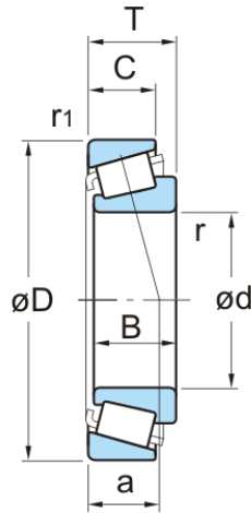
■ mounting dimensions
