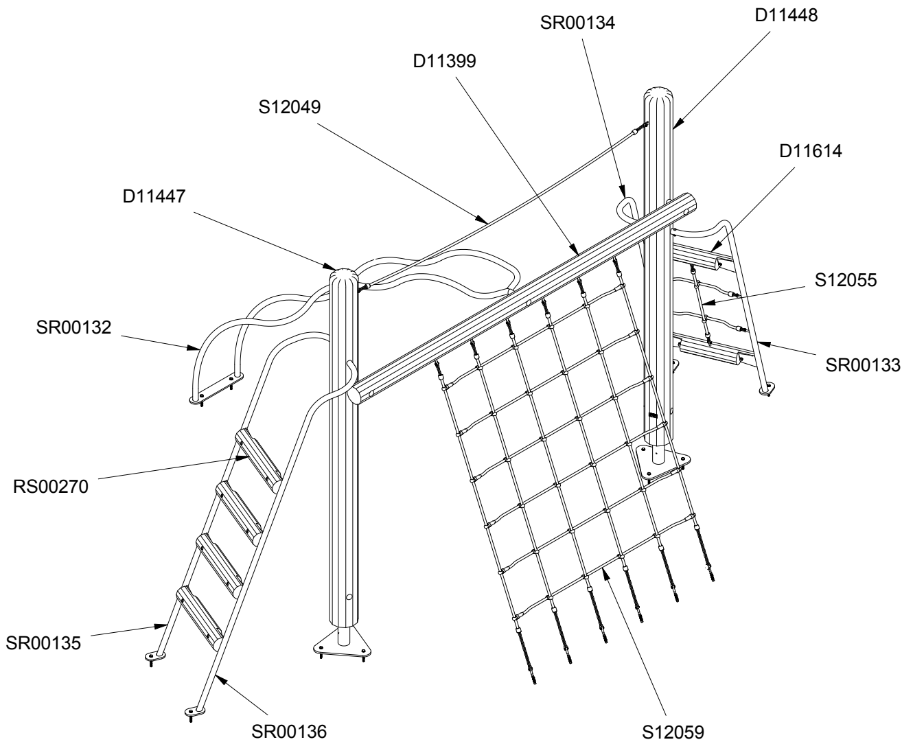
Parts List
