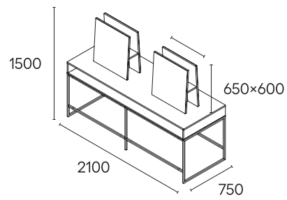
MESA 4S ISLAND
