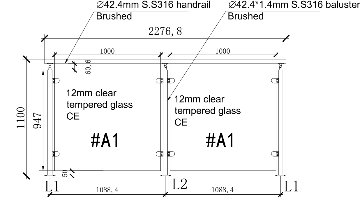
(EL) 2-ELEVATION SCALE: 1:1
