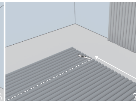
Step 7: Cut the acoustic panel into the remaining width.
