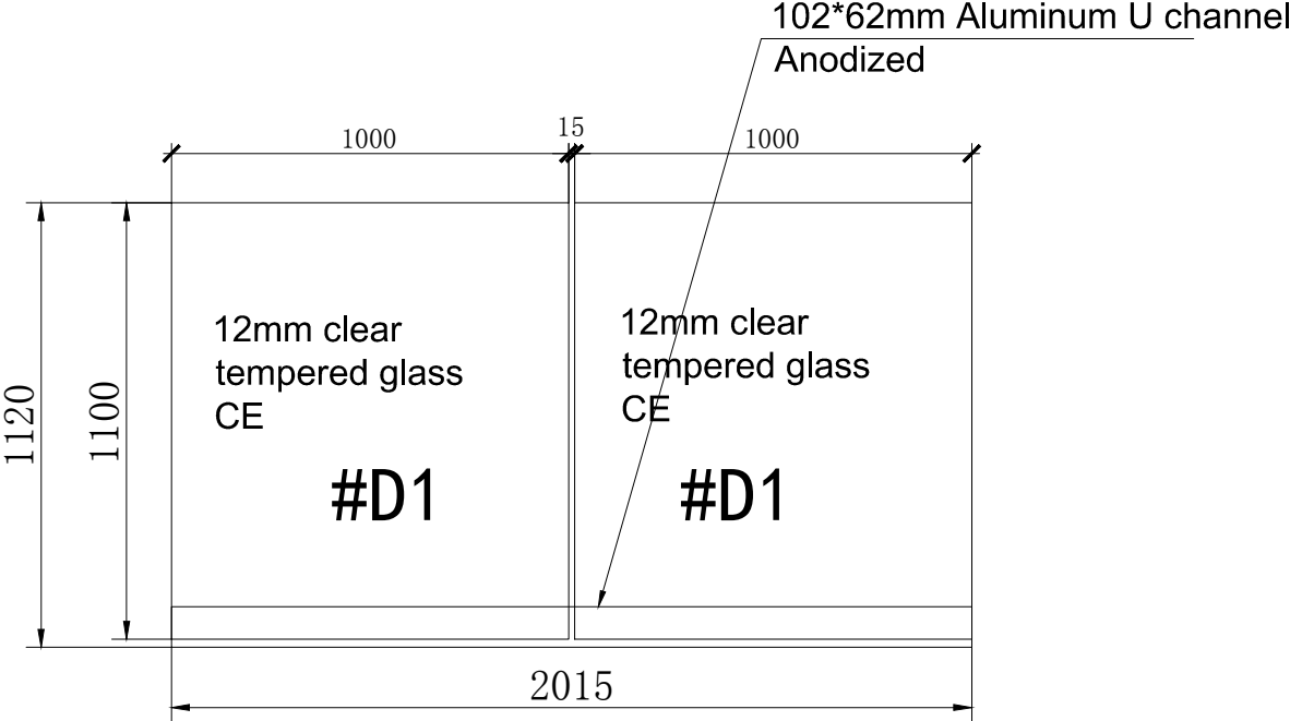
(EL) 14-ELEVATION SCALE: 1:1
