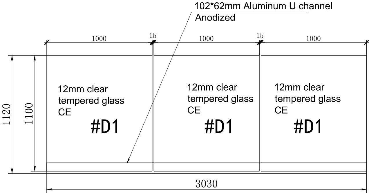
(EL) 15-ELEVATION SCALE: 1:1
