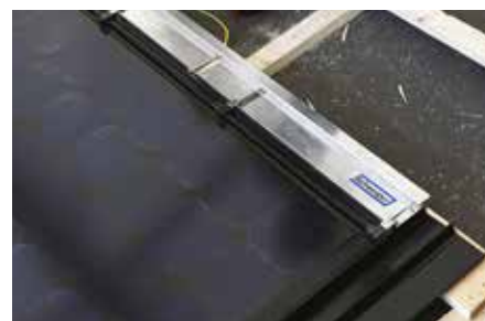
3 Fix the next rows of mounting clamps using the mounting gauge.
