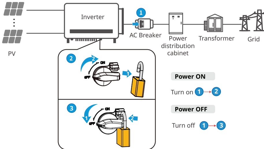
The DC switch locking hole is for Australia only.
