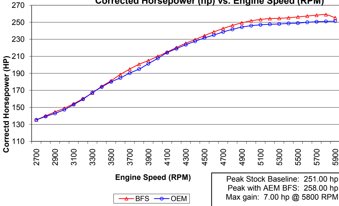
Corrected Horsepower (hp) vs. Engine Speed (RPM)
